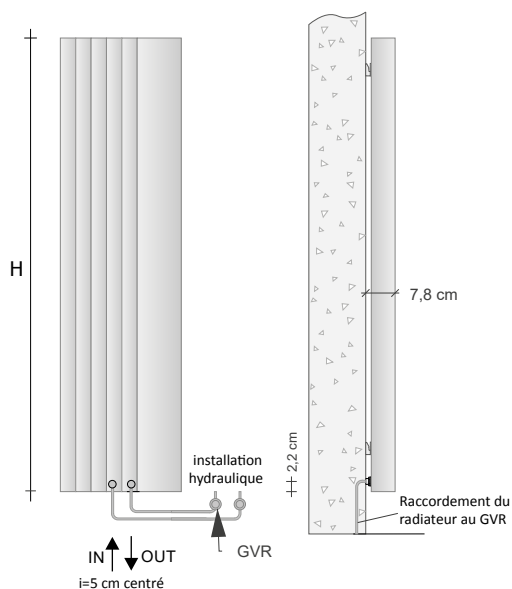
Version HYDRAULIQUE
