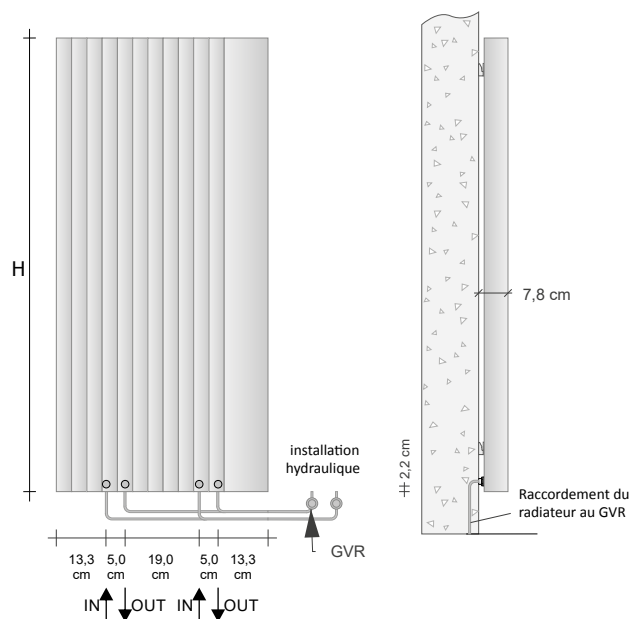
Version HYDRAULIQUE
