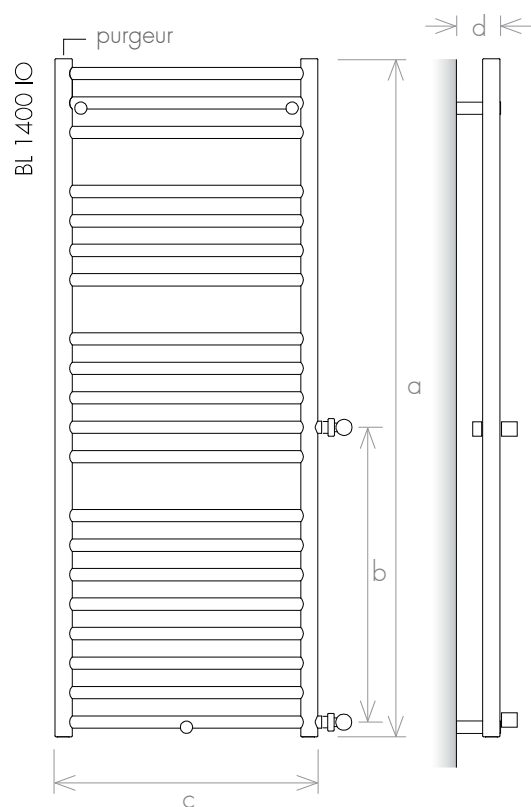
BL1400 IO (in&out) - raccordement latéral
