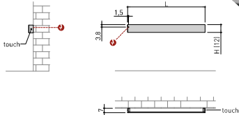
TOWEL BAR horizontal
