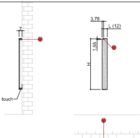
TOWEL BAR vertical
